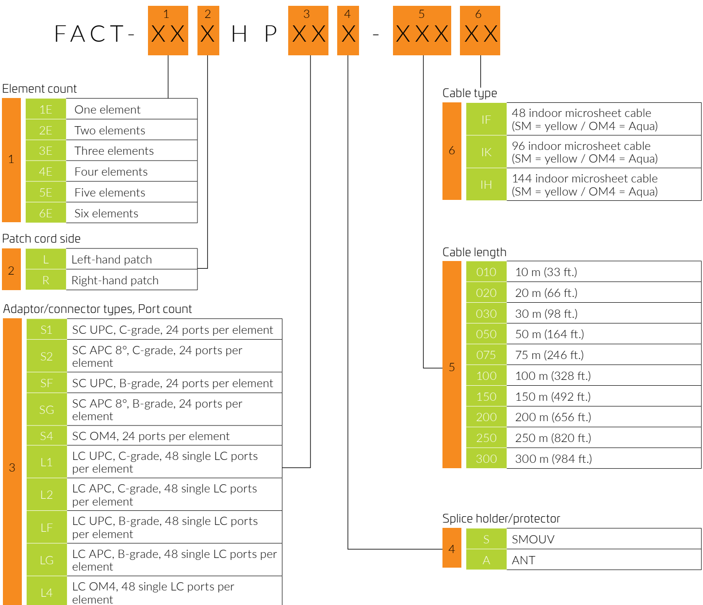
Figure 9: Two-element pre-cabled chassis with 96f. indoor microsheet cable and right-side patching
