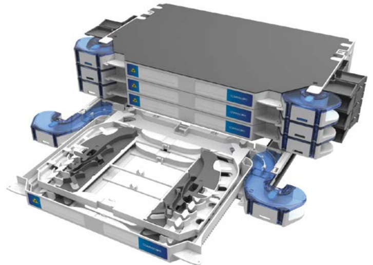
Figure 2: Four element universal FACT NG4 chassis
