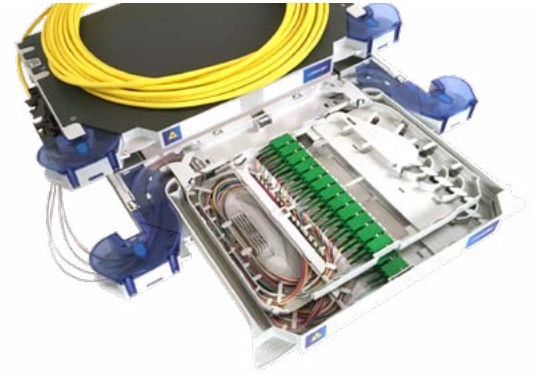
Figure 9: Two-element pre-cabled chassis with 96f. indoor microsheet cable and right-side patching
